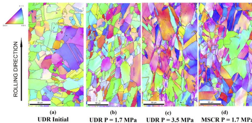
FIG. 8. Inverse pole figure (IPF) maps of (a) UDR sample, (b) UDR sample shock-loaded at P = 1.7 MPa, (c) UDR sample shock-loaded at P = 3.5 MPa, and (d) MSCR sample shock-loaded at P = 1.7 MPa.
