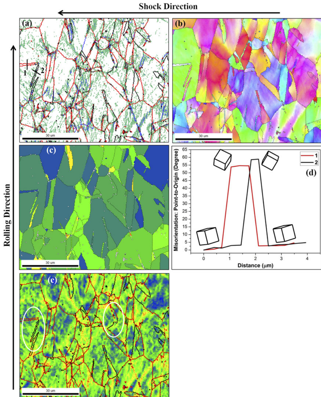
FIG. 13. Plots for UDR sample deformed at P = 3.5 MPa. (a) Grain boundary map. The red line indicates the HARB, black line twin ( \Sigma 3 CSL) boundary, green-line VLAB ( 2-5^\circ ), and blue-line LAGB ( 5-15^\circ ). (b) Rotated IPF map showing plane orientation perpendicular to shock or parallel to normal plane. For color code, refer to Fig. 8. (c) Grain average misorientation map showing the average misorientation in various grains. The color scale is from minimum blue to maximum red with cutoff of 5^\circ misorientation. The misorientation line profile along lines 1 and 2 in (a) is shown in (d). (e) KAM map showing the local misorientation inside the grains. The line represents boundary type as in (a). The white ellipse marks the region showing different boundary type surrounding twins. Note the KAM around the different boundaries surrounding the twin. All scale bars in the maps are 30 \mu\text{m} in size.
