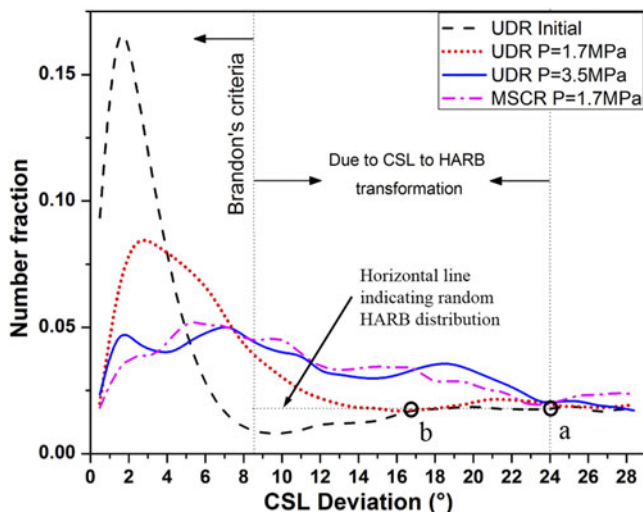
FIG. 16. Twin ( \Sigma 3 CSL) deviation plot obtained from EBSD data for UDR sample, UDR sample shock-loaded at P = 1.7 MPa and at P = 3.5 MPa, and MSCR sample at P = 1.7 MPa.
