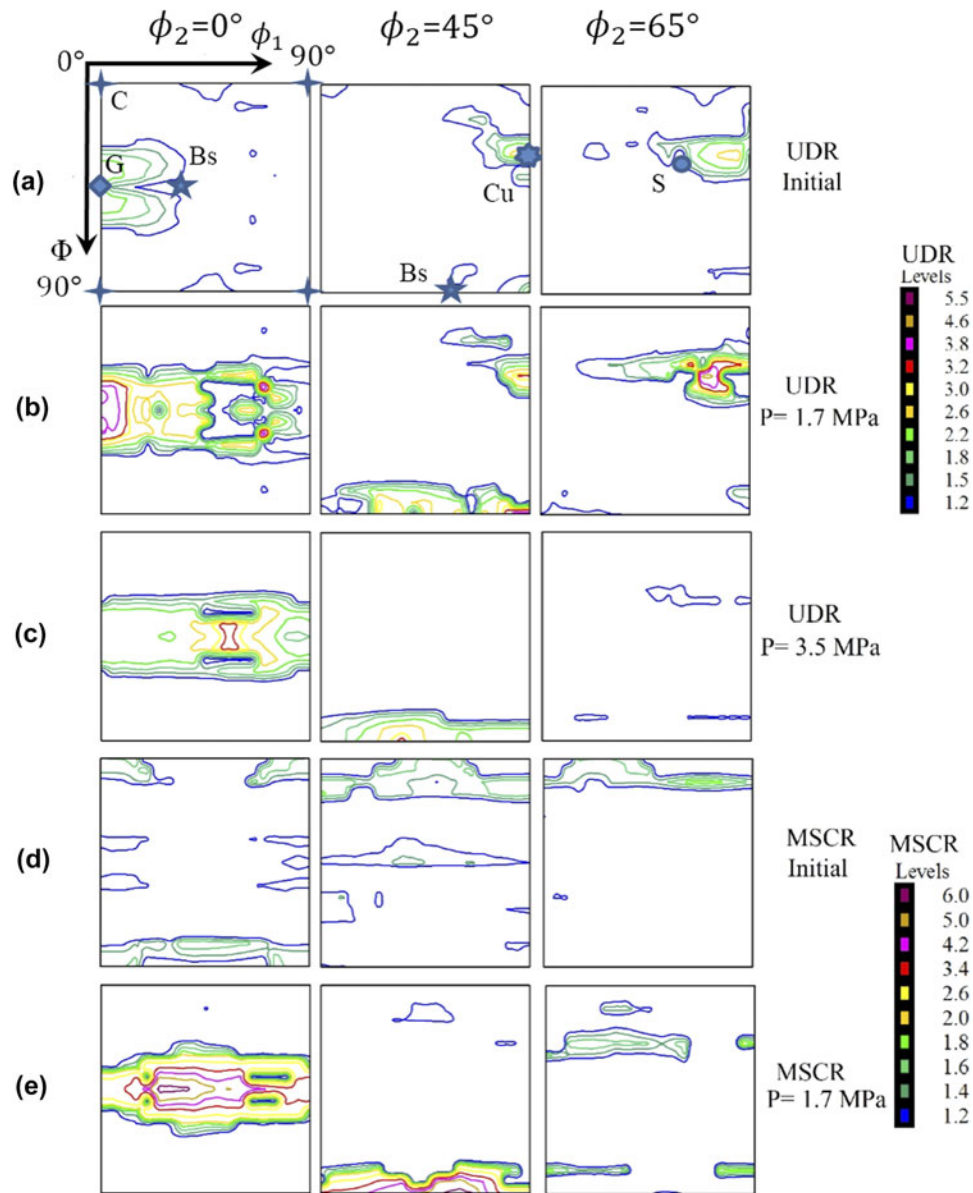
FIG. 5. Selected ODF sections \phi_2 = 0^\circ , 45^\circ , and 65^\circ for the (a) UDR sample, (b) UDR sample subjected to shock deformation at P = 1.7 MPa, (c) UDR sample shock-loaded at P = 3.5 MPa, (d) MSCR sample, and (e) MSCR sample shock-loaded at P = 1.7 MPa.
